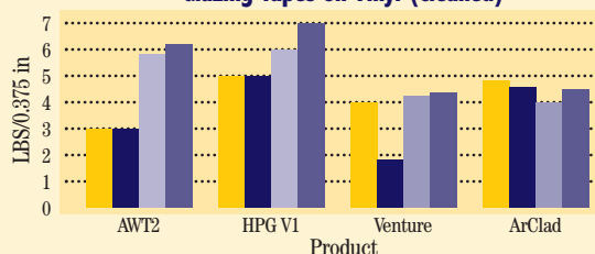
Adhesion Properties of PE Foam Glazing Tapes on Vinyl (Cleaned)
